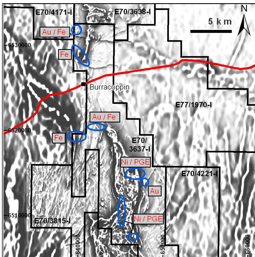
Burracoppin Project, 1 st VD Magnetic Image and Drill Targets
