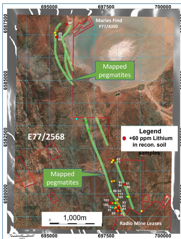
Figure 3. Bullfinch North, Mapped Pegmatite Occurrences with Li ppm
